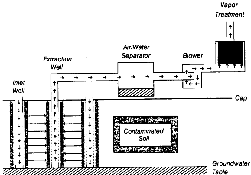
Figure 1. Soil vapor extraction system.
